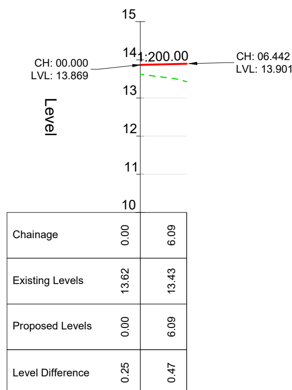
ROAD 4 - LONGSECTION SCALE: H 1:500,V 1:100
