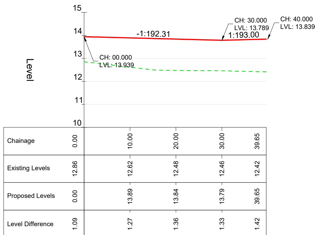
ROAD 3 - LONGSECTION SCALE: H 1:500,V 1:100
