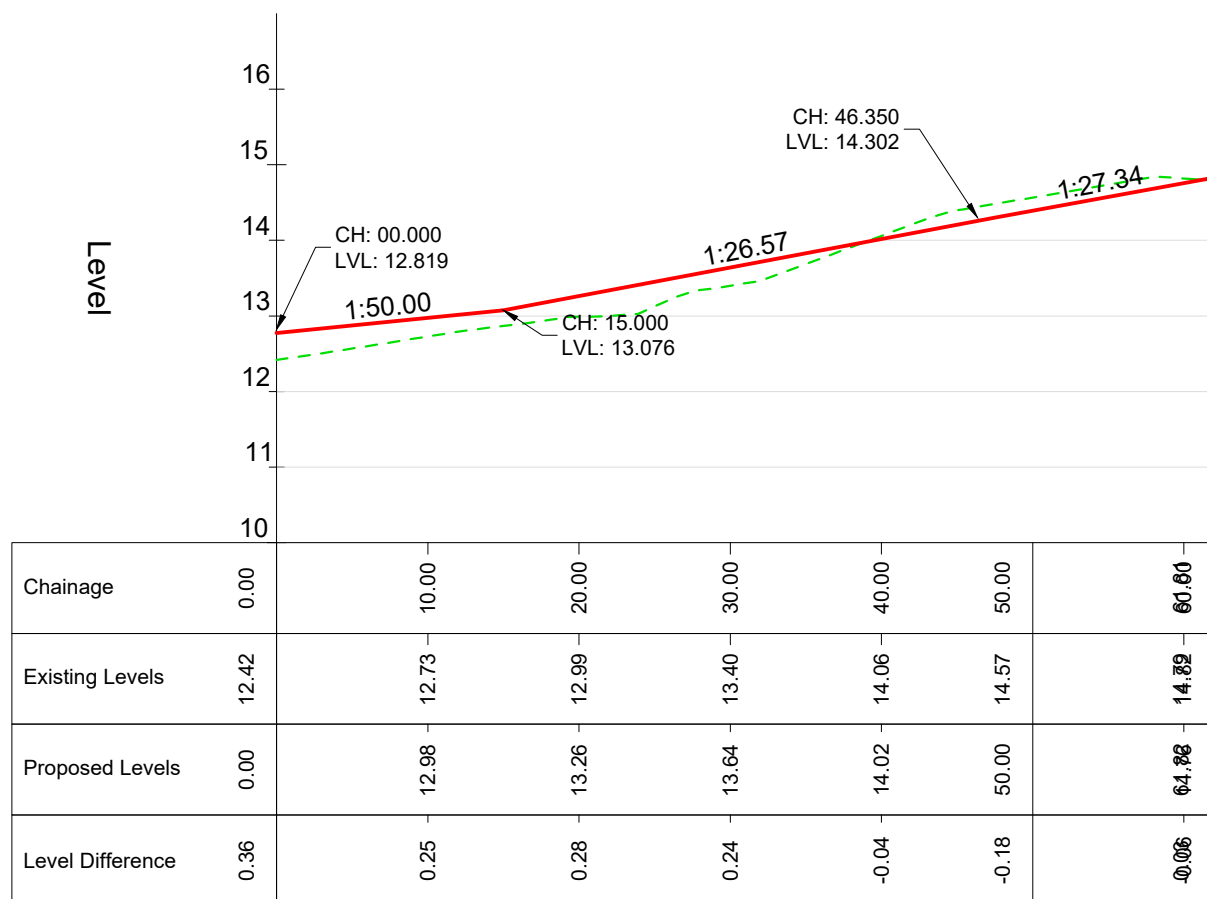
ROAD 2 - LONGSECTION SCALE: H 1:500,V 1:100
