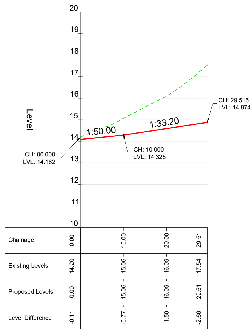
ROAD 5 - LONGSECTION SCALE: H 1:500,V 1:100
